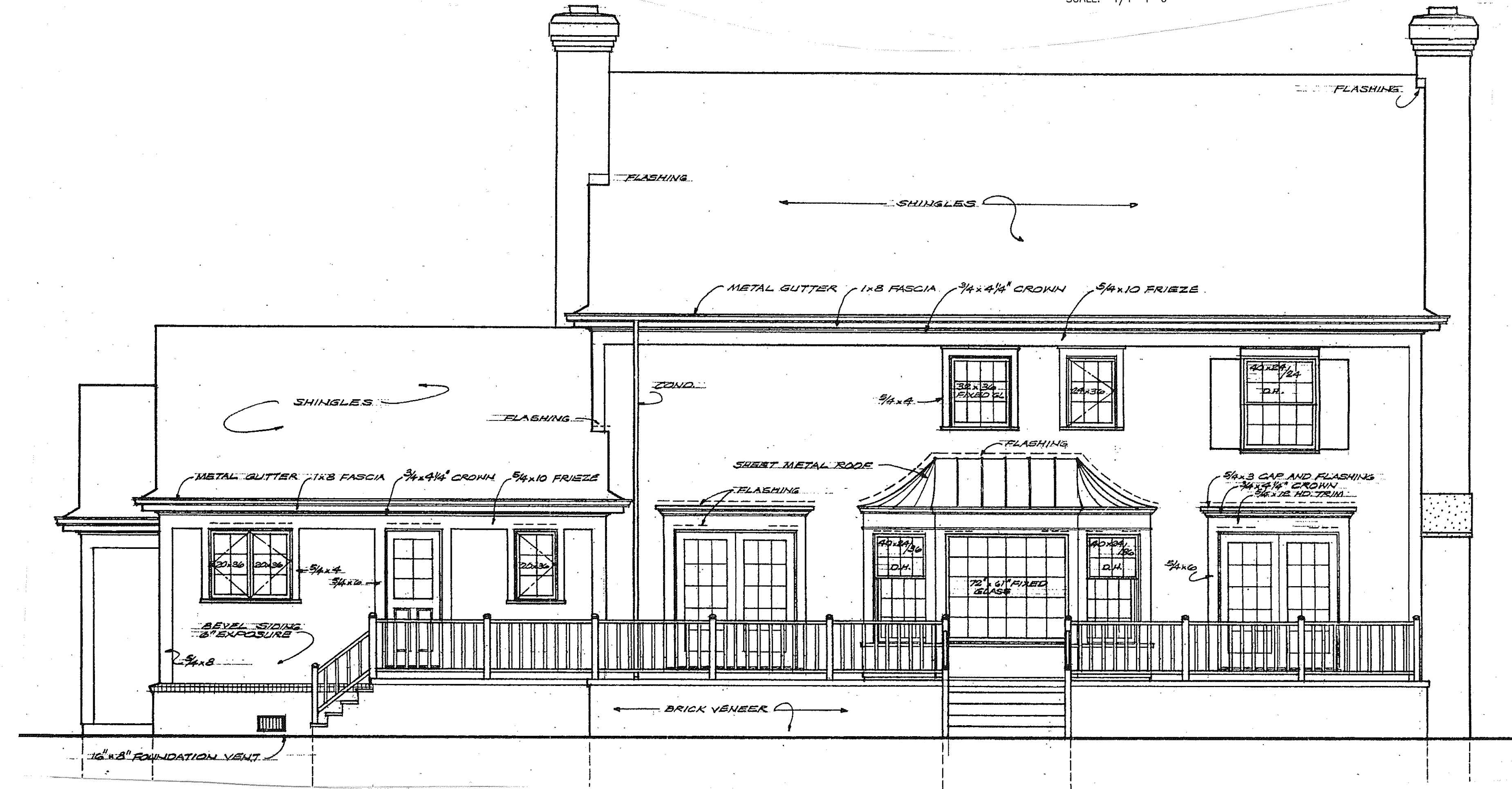
FRONT ELEV.
