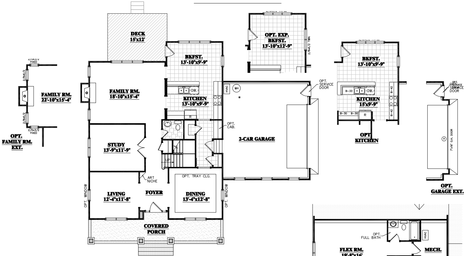
First floor Plan — Elev. C
