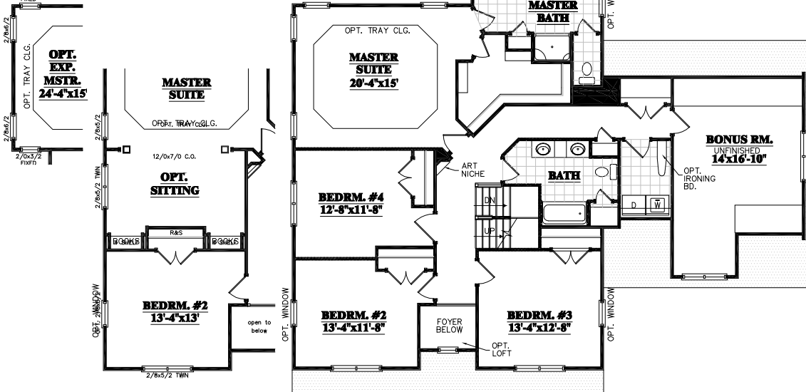
Second floor Plan — Elev. C
