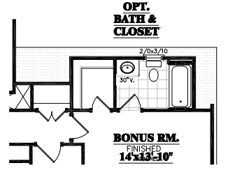
Third floor Plan OPTIONAL
